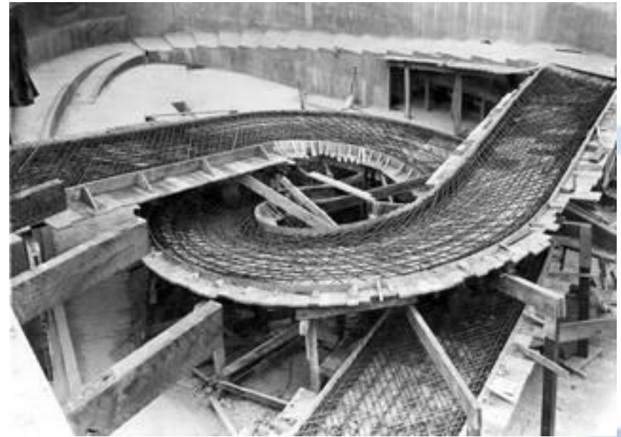
Penguins pool designed by Arup
